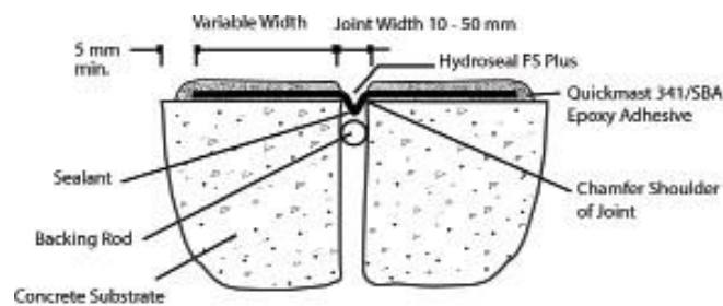
Expansion & Contraction Joints
