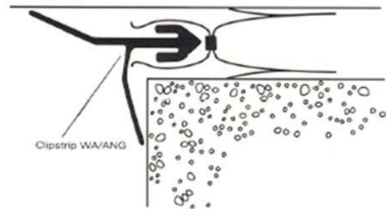
WALL - CORNER JOINT DETAIL
