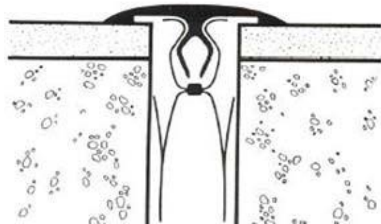
FLOOR - JOINT DETAIL
