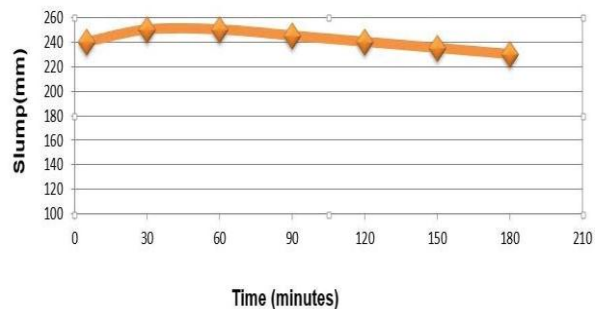
CEMII OPC 42.5 & Cement replacements 1.7% Hyperplast 150+
